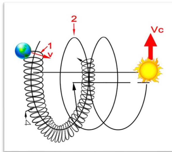
Archimedes' Spiral
