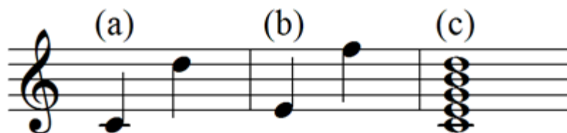
(a) — large nona, (b) — small nona, (c) — nonaccord, in it the upper note is the non tone
